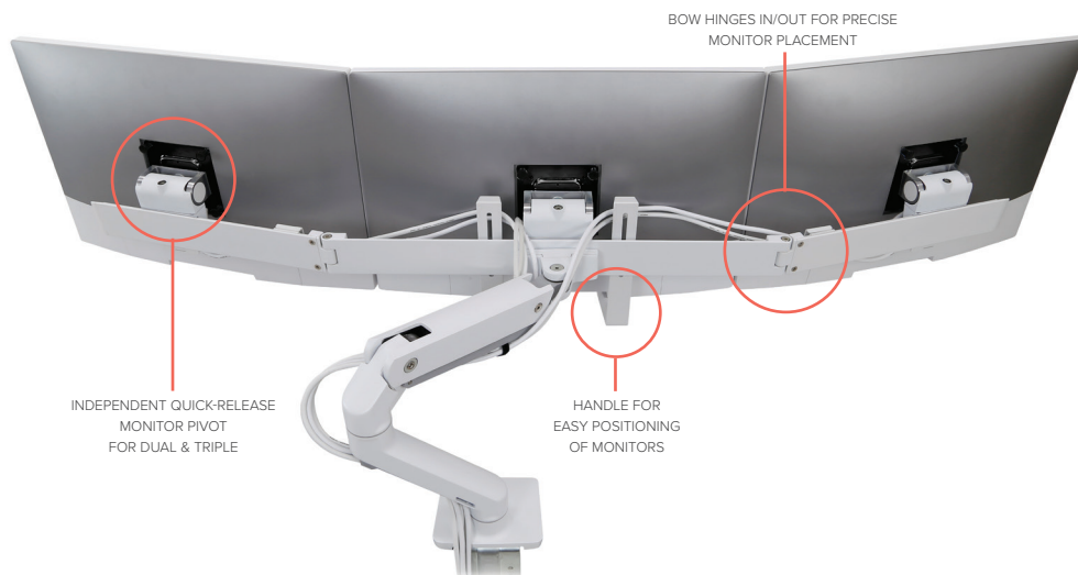
HX DESK MONITOR ARM WITH HX TRIPLE MONITOR BOW KIT
