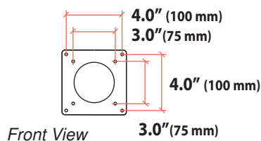
Monitor Mount
