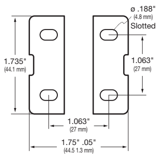
Single Pivot w/ P/L Interface
