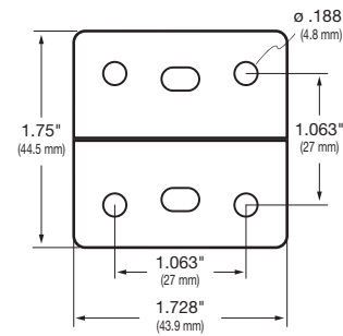
Double Pivot w/ P/L Interface
