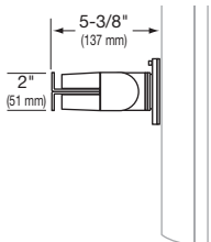
Double Pivot with P/L
