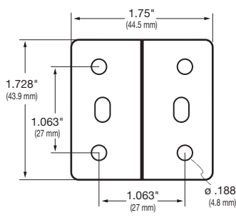
Keyboard/Laptop Pivot Interface
